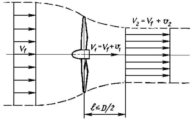
Fig. 1.4. Flow profile near propeller
