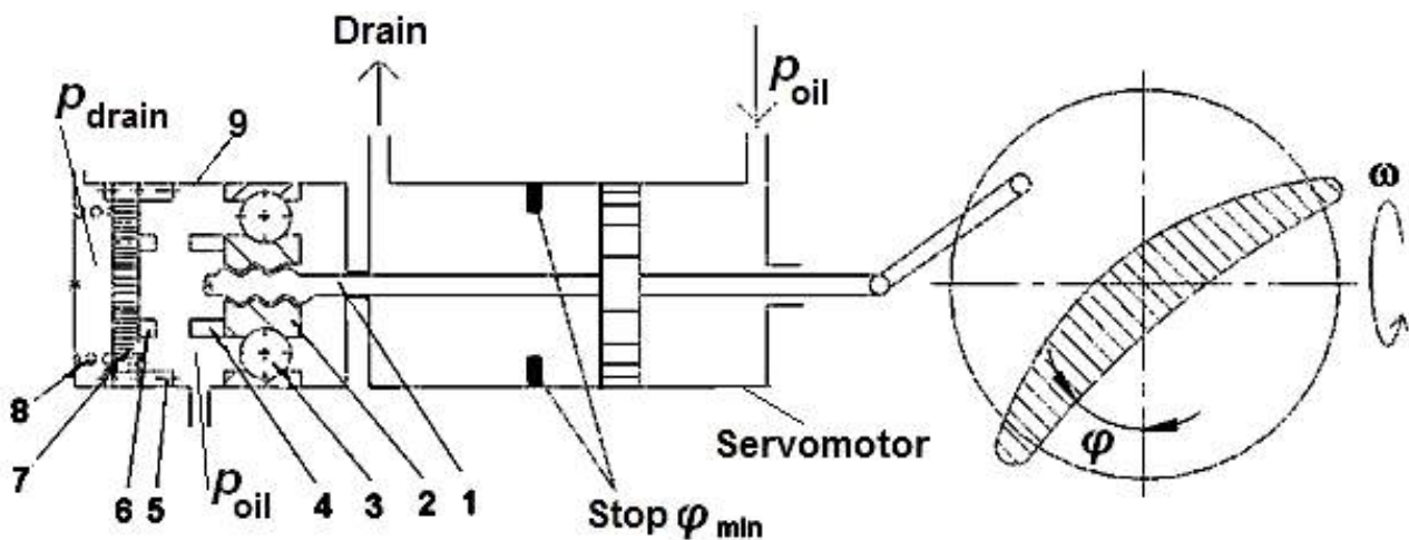
Fig. 3.3. Mechanical pitch stop: 1 – drive screw; 2 – nut; 3 – bearing; 4, 6 – face splines; 5 – splines on the cylindrical surface; 7 – piston; 8 – spring; 9 – cylinder of MPS
