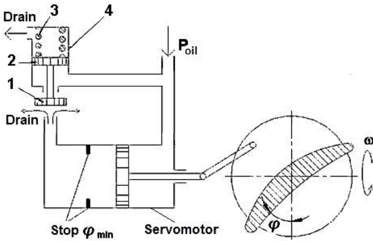
Fig. 3.2. Hydraulic pitch stop: 1 – valve; 2 – piston; 3 – spring; 4 – cylinder of hydraulic pitch stop
