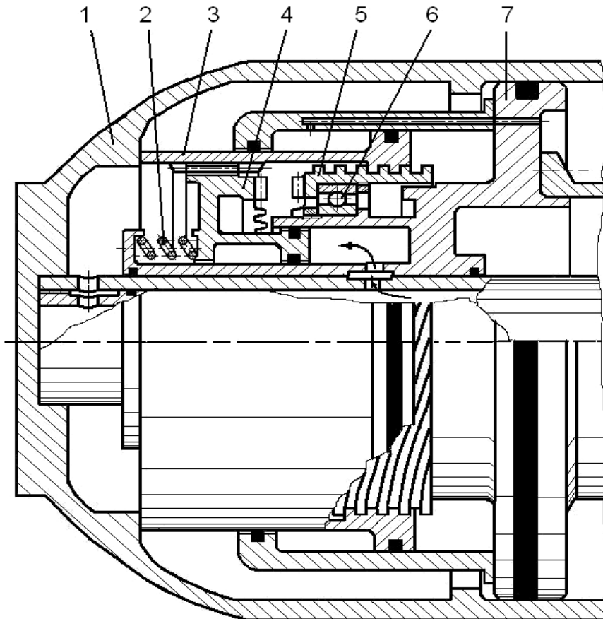
Fig. 4.10. Mechanical pitch stop:
