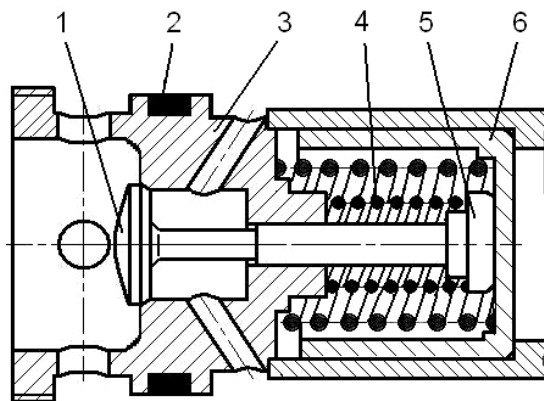
Fig. 4.9. Hydraulic pitch stop:
