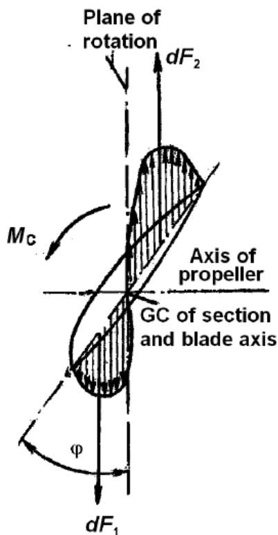
Fig. 1.9. Diagram of transversal components of centrifugal forces in blade section
