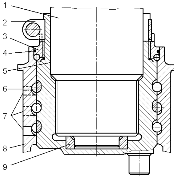
Fig. 4.6. Blade fixing to hub casing:
