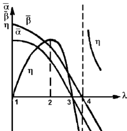
Fig. 1.6. Aerodynamic performances of propeller at constant blade angle
