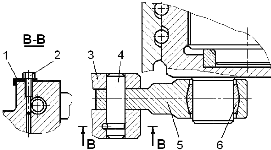
Fig. 4.7. Junction between connecting rod, cross bar and pin of cartridge:
