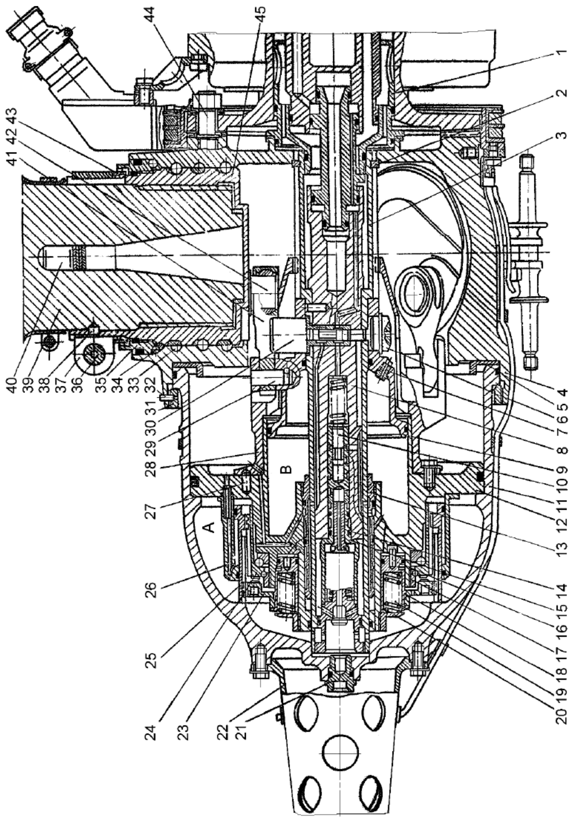
Fig. 6.1. Hub of aircraft propeller AV-681
