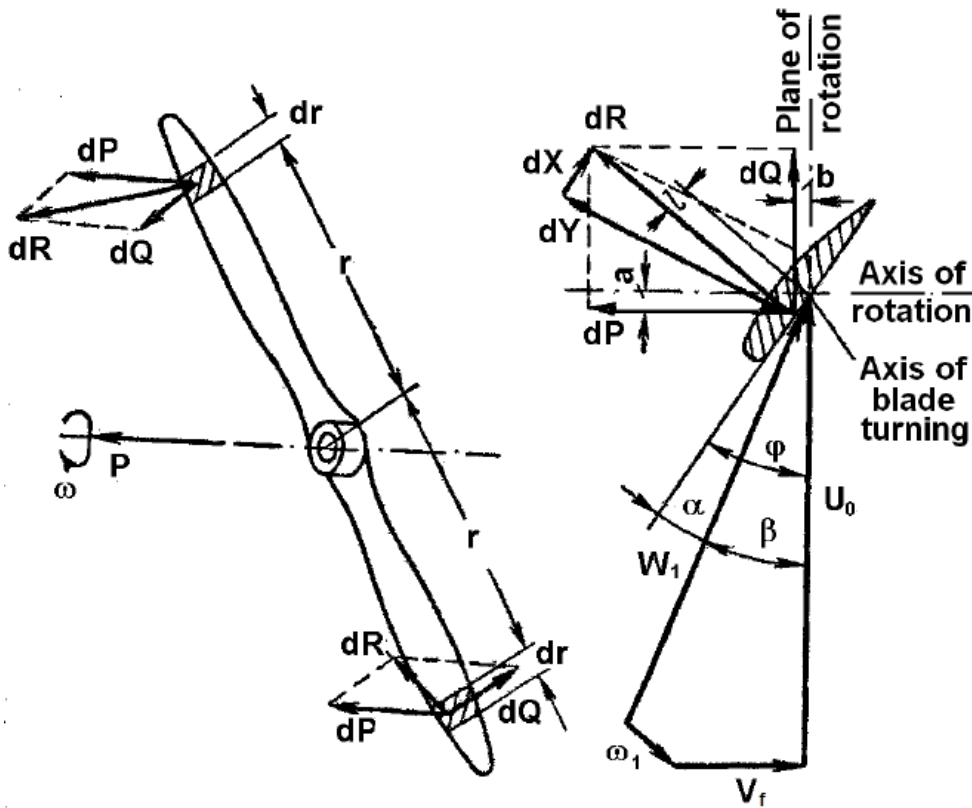
Fig. 1.5. Aerodynamic forces acting a blade element
