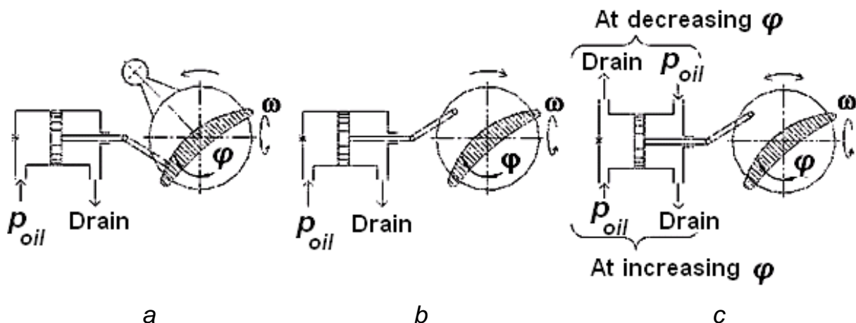
Fig. 2.2. Schemes of hydraulic propellers: a – direct action ( \varphi decreases); b – back action ( \varphi increases); c – double action
