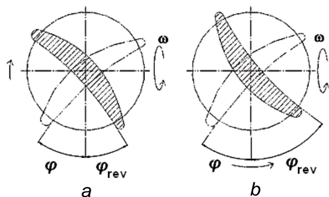
Fig. 2.4. Methods of blades driving to reverse position:
