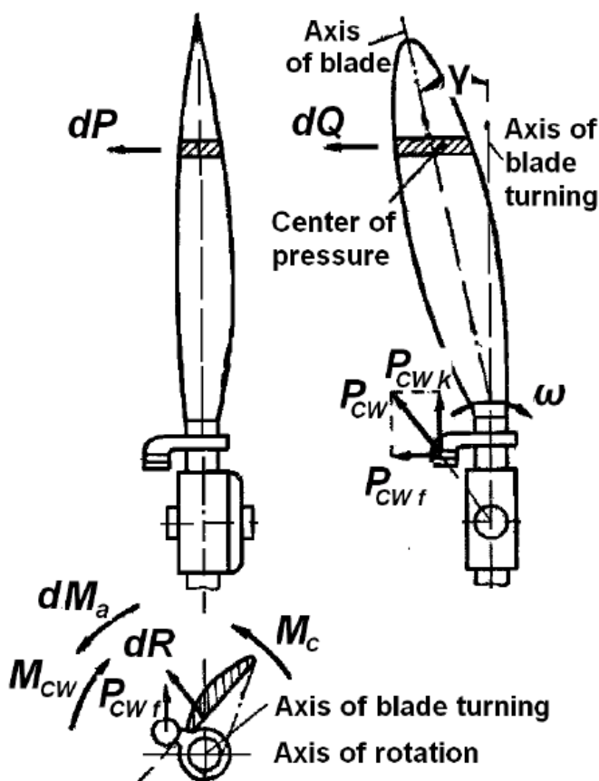
Fig. 2.1. Aeromechanical propeller
