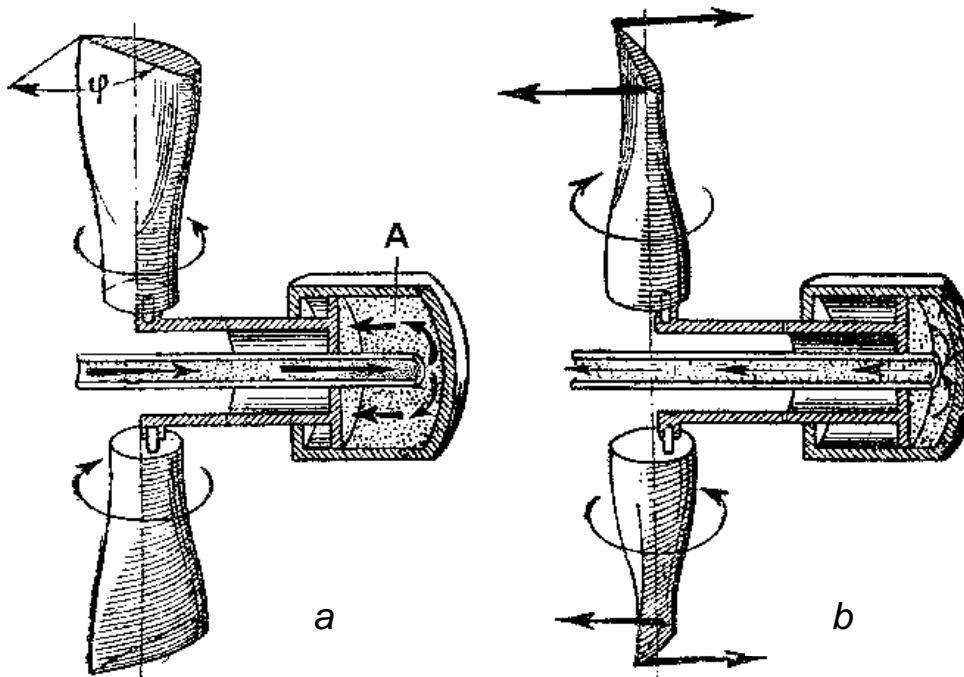
Fig. 4.4. Operating of hub of hydraulic VPP that operates on back-action scheme:
