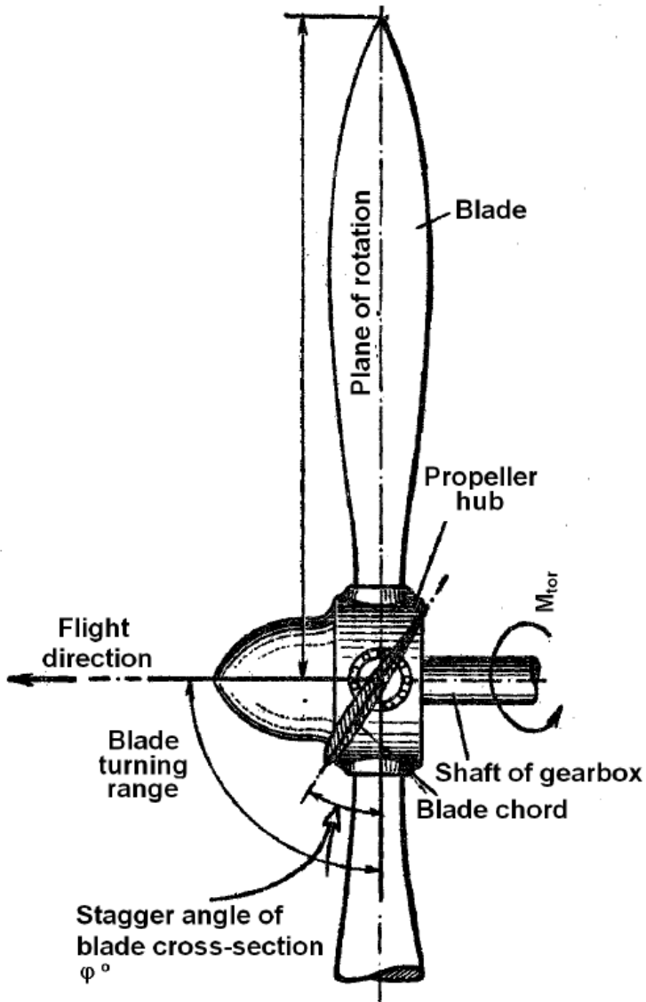
Fig. 1.1. Aircraft propeller
