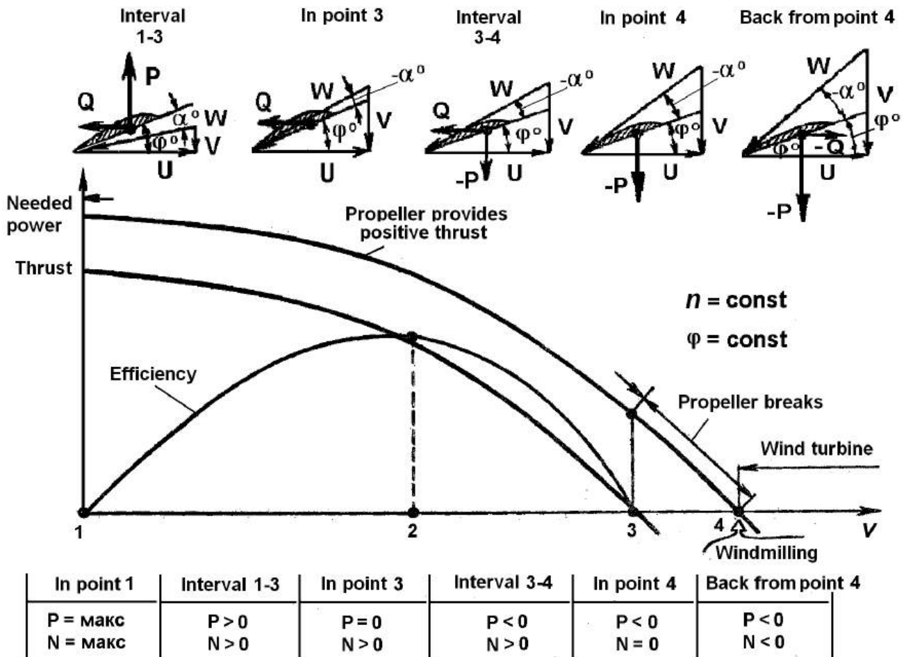
Fig. 1.7. N_p , P and \eta vs flight velocity at constant rotation speed and constant blade angle
